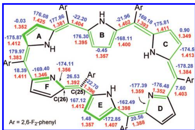
Figure 9. Detailed structural data for the Möbius structure of 2b from Figure 8. The conjugated 28 \pi -electron circuit is indicated in green, along with bond lengths ( \text{\AA} ) are indicated in red and dihedral angles (deg) in blue.
