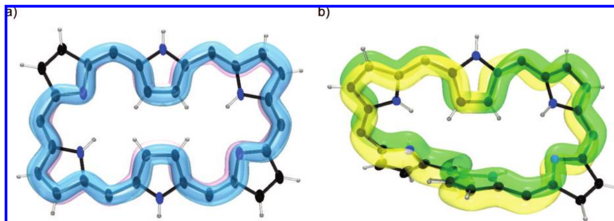
Figure 1. Topological models of [28]hexaphyrins: (a) planar rectangular conformation of Hückel topology; (b) twisted Möbius topology.
