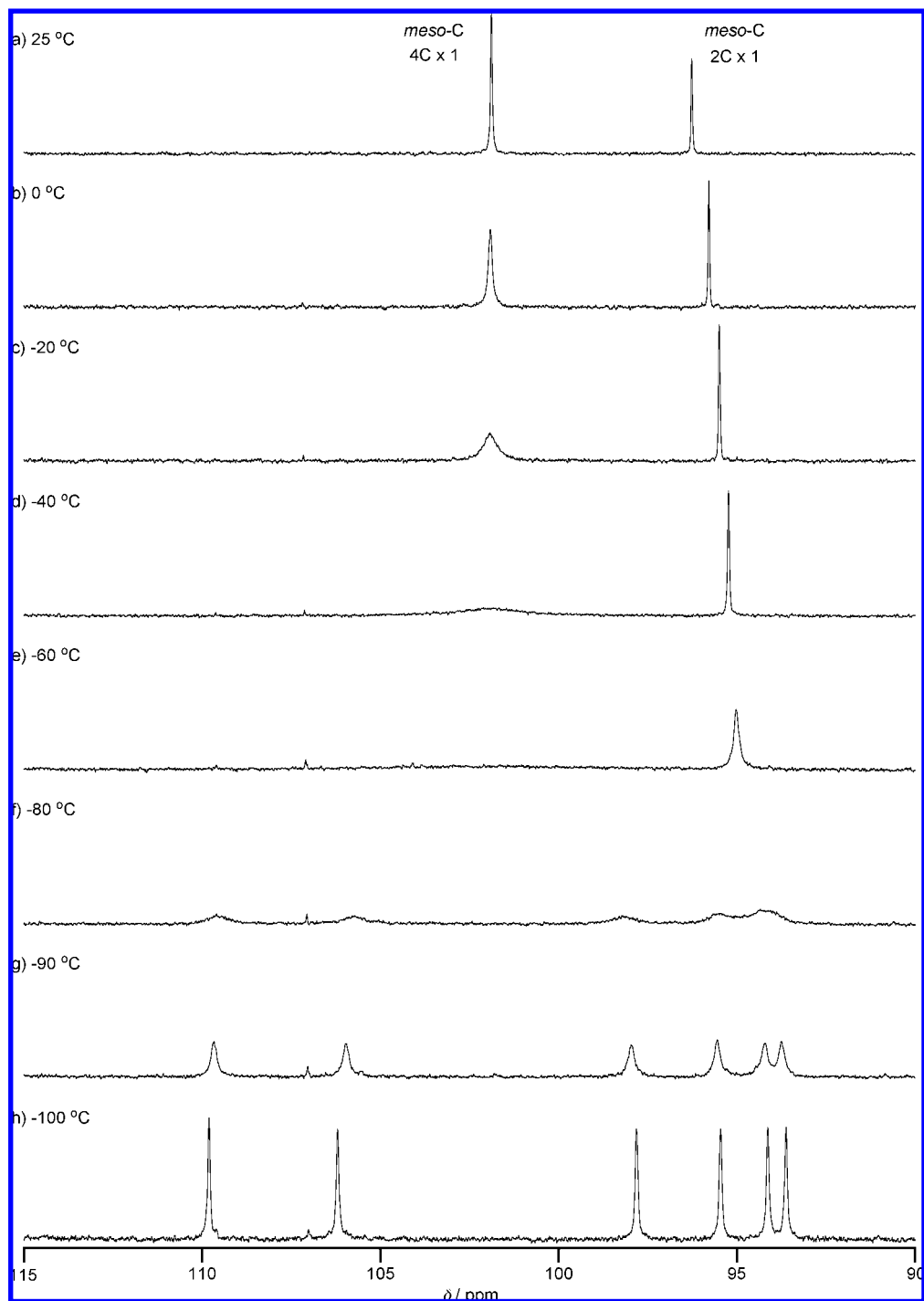
Figure 3. Variable-temperature ^{13}\text{C} NMR spectra of meso - ^{13}\text{C} -enriched 2a in \text{THF-}d_8 from 25 to -100 °C.
