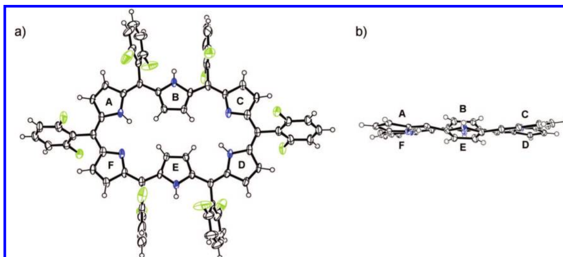
Figure 7. X-ray structure of 2b obtained from CHCl 3 / n -heptane: (a) top view; (b) side view. The thermal ellipsoids are scaled to the 50% probability level. In the side view, the meso -aryl substituents have been omitted for clarity.
